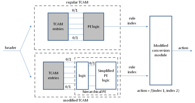
(b) Suggested In/Out TCAM architecture. It includes a regular TCAM and a modified TCAM. In the modified TCAM, each range is encoded separately, and the regular PE is replaced by a hierarchical PE that is used to select the first matching range. Finally, the action is selected based on the indices sent by the two TCAMs.
