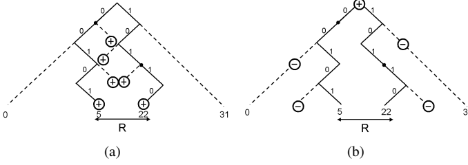
Fig. 3. Two encoding schemes of the range R = [5, 22] = \{00101, \dots, 10110\} from Example 4. Fig. 3(a) presents the encoding of R itself as a union of several prefix ranges. The six plus signs represent the six TCAM entries in this encoding. Fig. 3(b) demonstrates the alternative encoding of R in which we first negatively encode (with out entries) the complement of R and then add an additional in entry that matches R itself. Again, the five signs represent the five entries of this encoding. For any W -bit range R , one of these two encodings has at most W entries.
