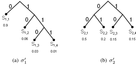
Fig. 2. Illustration of a second encoding scheme C_D = (\sigma'_1, \sigma'_2) with an improved success probability P_{success}(L = 3, C_D) = 0.9 .
